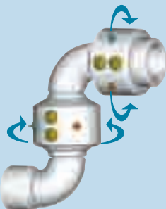
Style 50 2 planes of rotation
