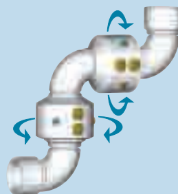
Style 70 2 planes of rotation
